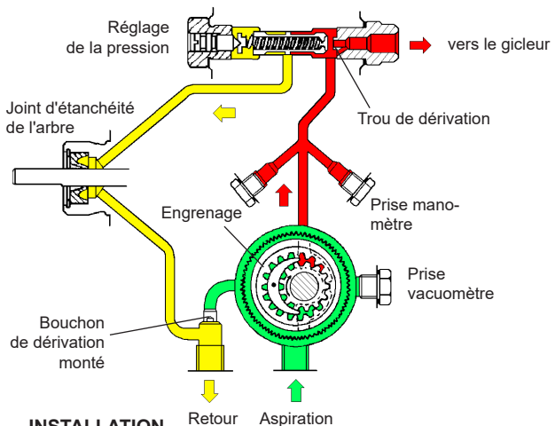
INSTALLATION BITUBE
